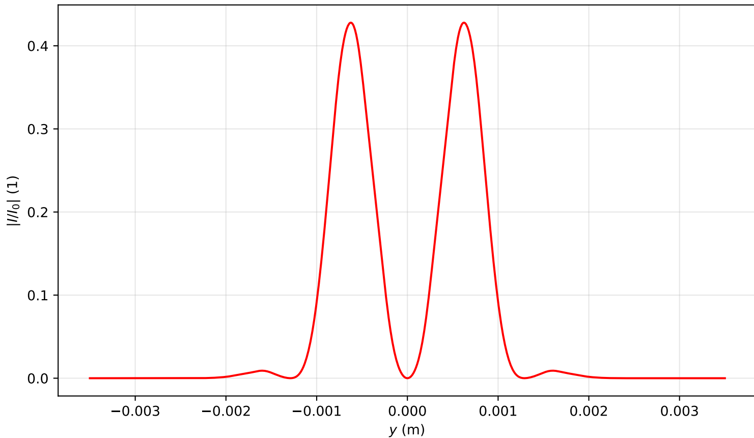
Intensity profile I(x=0, y, z=1.513)/I_0 , P_{in}=5.0P_{cr} , artificial time
